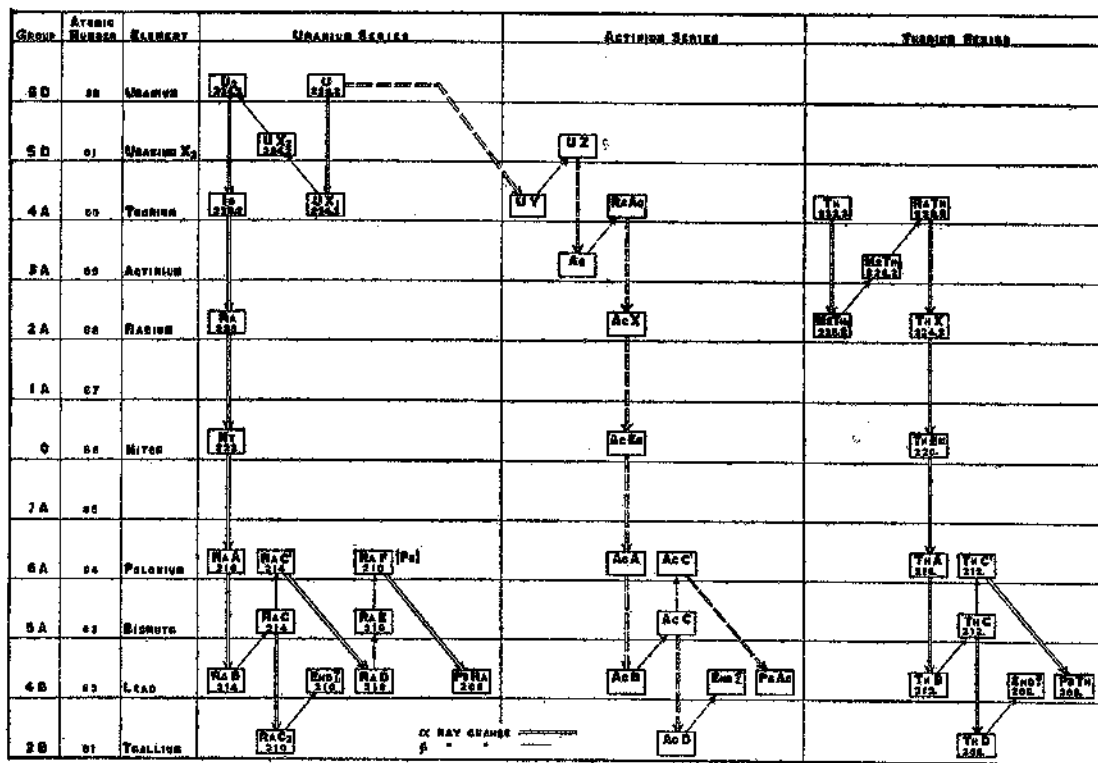
FIG. 1. TRANSFORMATIONS OF THE RADIOACTIVE ELEMENTS. The \alpha and \beta changes of the radioactive elements. Note that the atoms of even atomic number are more numerous than those of odd atomic number. Thus there are 32 of the former class to 11 of the latter.
